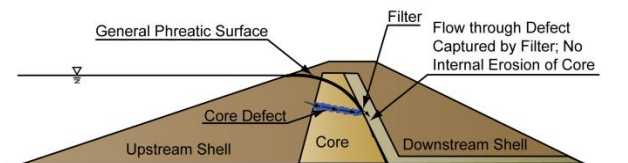
Figure 1: Filter collecting flow through core defect.
