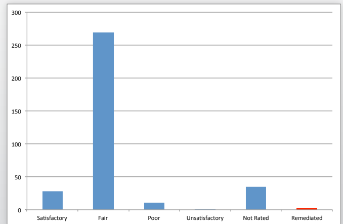
2015 Condition Rating & Number Remediated of State-Regulated High Hazard Potential Dams.
